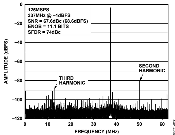
Figure 27. AD9627-125 Single-Tone FFT with f_{IN} = 337 MHz
