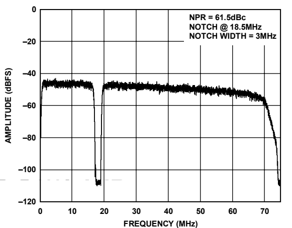
Figure 38. AD9627-150 Noise Power Ratio (NPR)
