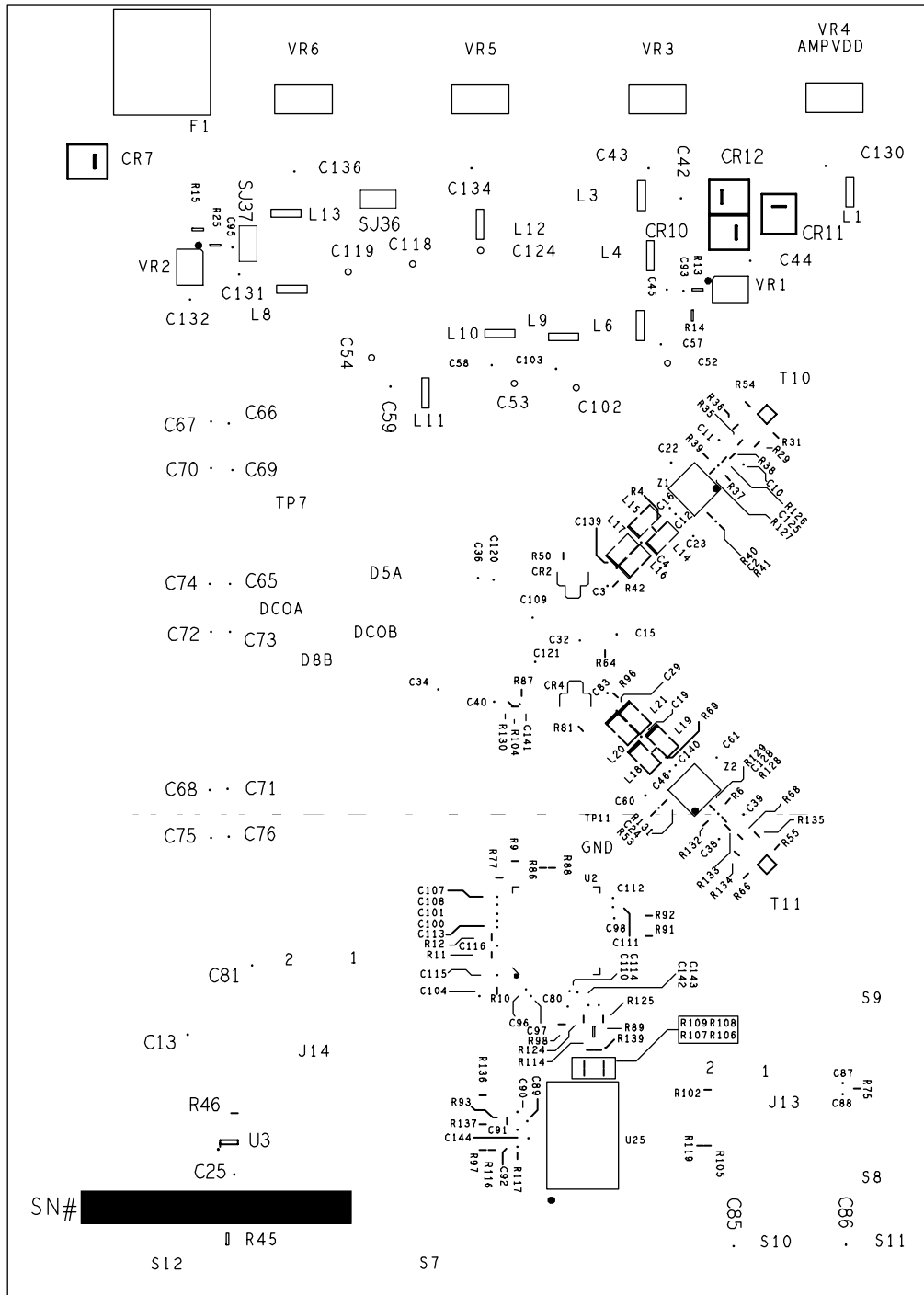
Figure 92. Evaluation Board Layout, Silkscreen, Secondary Side
