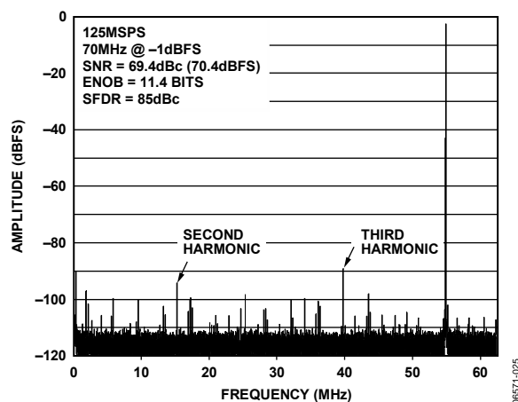
Figure 25. AD9627-125 Single-Tone FFT with f_{IN} = 70 MHz
