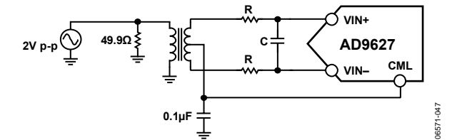
Figure 47. Differential Transformer-Coupled Configuration
