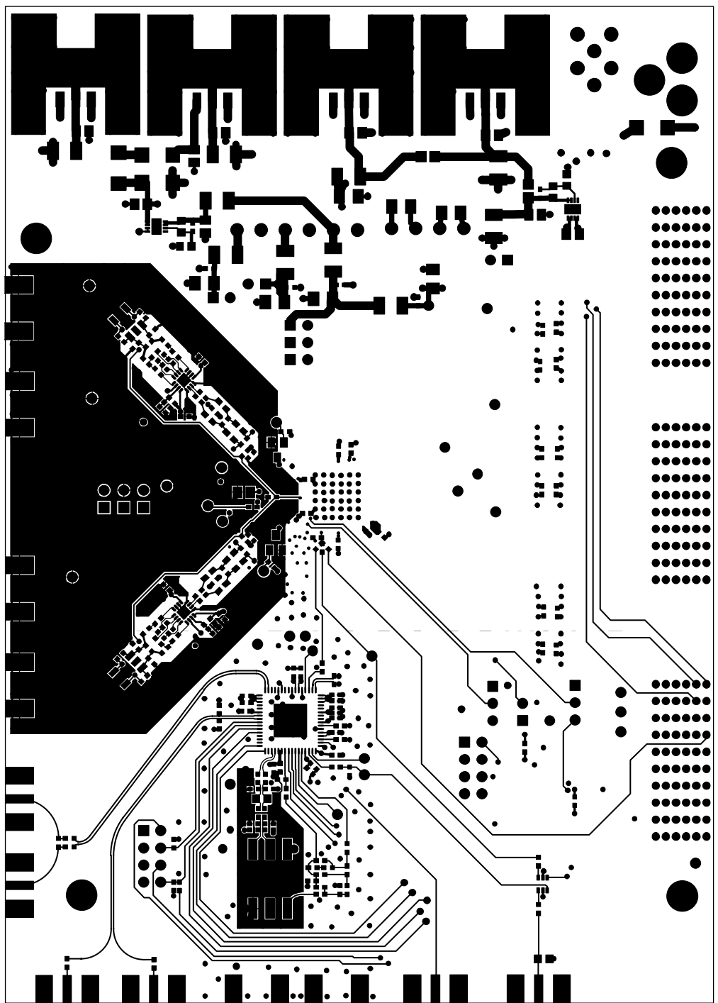
Figure 90. Evaluation Board Layout, Secondary Side (Mirrored Image)
