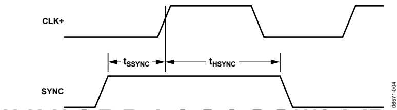
Figure 4. SYNC Input Timing Requirements
