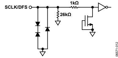
Figure 12. Equivalent SCLK/DFS Input Circuit
