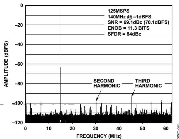
Figure 26. AD9627-125 Single-Tone FFT with f_{IN} = 140 MHz
