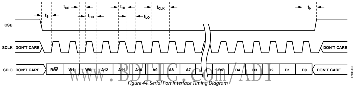
Figure 44. Serial Port Interface Timing Diagram
