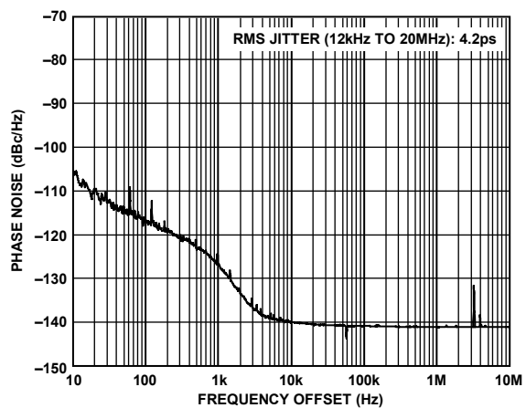
Figure 11. Additive Phase Noise at HSTL Output Driver, \text{SYSCLK} = 500 \text{ MHz} ( \text{SYSCLK PLL Disabled} ), f_{\text{REF}} = 10.24 \text{ MHz} , f_{\text{OUT}} = 20.48 \text{ MHz} , \text{DPLL Loop BW} = 1 \text{ kHz}
