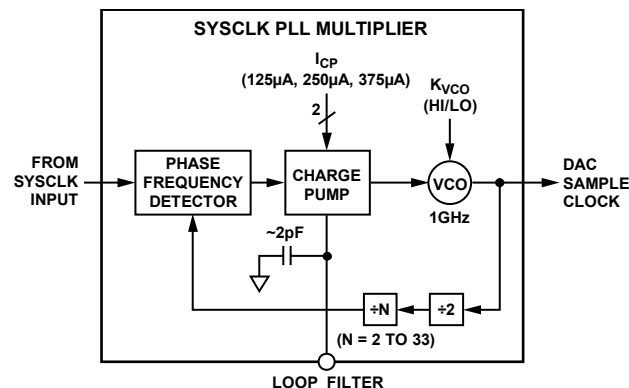
Figure 43. Block Diagram of the SYSCCLK PLL
