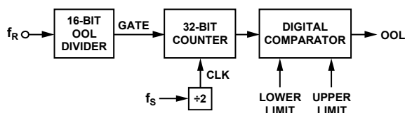
Figure 32. Reference Monitor
