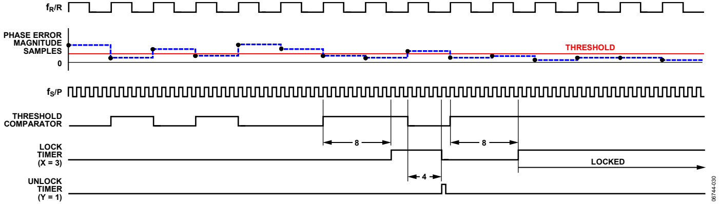
Figure 30. Lock/Unlock Detection Timing
