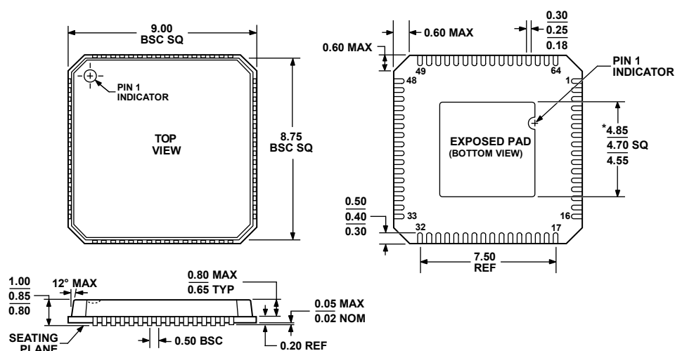
Figure 60. 64-Lead Lead Frame Chip Scale Package [LFCSP_VQ] 9 mm × 9 mm Body, Very Thin Quad (CP-64-1)
