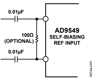
Figure 20. Reference Input
