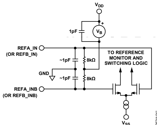
Figure 41. Reference Inputs
