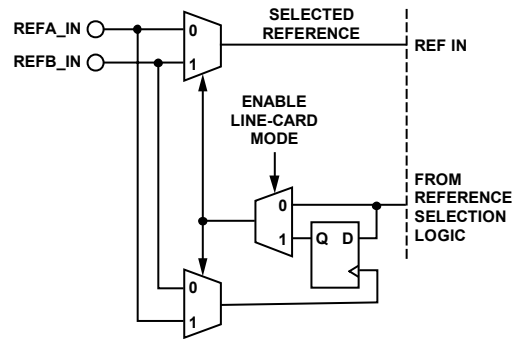
Figure 34. Reference Switchover Control Logic
