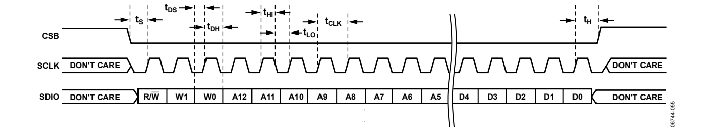
Figure 55. Serial Control Port Write: MSB First, 16-Bit Instruction, Timing Measurements
