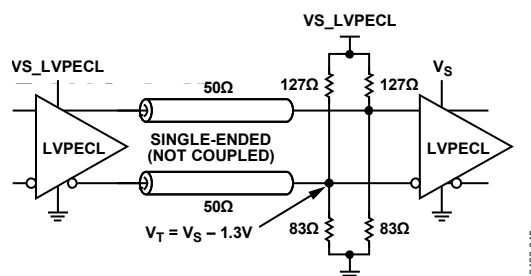
Figure 51. LVPECL Far-End Thevenin Termination
