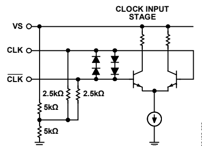
Figure 35. CLK Equivalent Input Circuit
