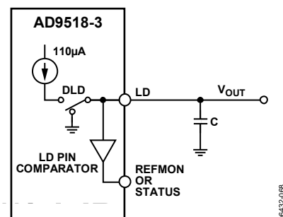
Figure 34. Current Source Digital Lock Detect
