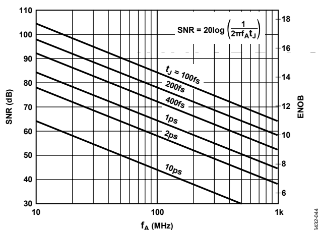
Figure 50. SNR and ENOB vs. Analog Input Frequency
