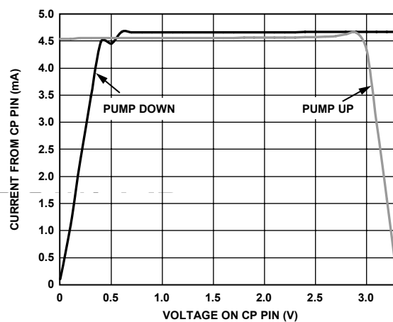
Figure 11. Charge Pump Characteristics @ V_{CP} = 3.3\text{ V}
