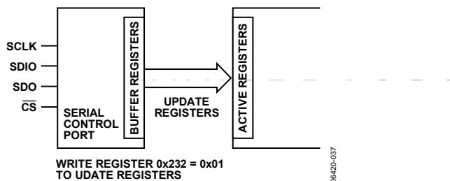
Figure 61. Relationship Between Serial Control Port Buffer Registers and Active Registers of the AD9516
