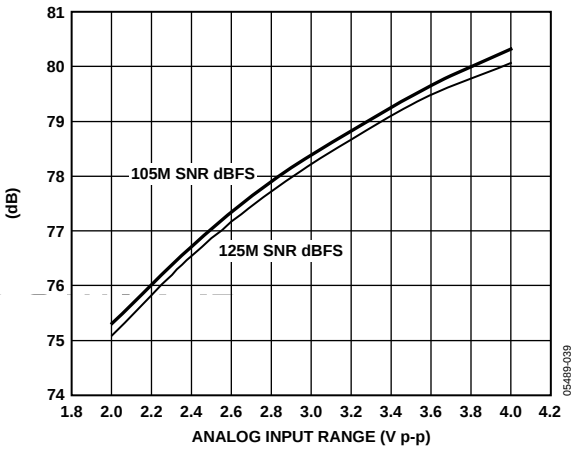
Figure 58. SNR vs. Analog Input Range, 2.3 MHz @ -30 dBFS
