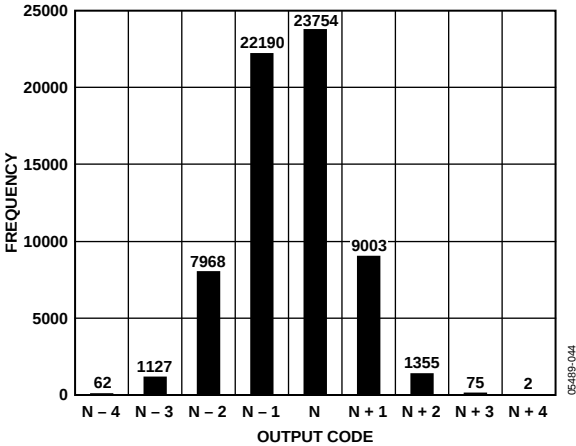
Figure 42. AD9445-125 Grounded Input Histogram
