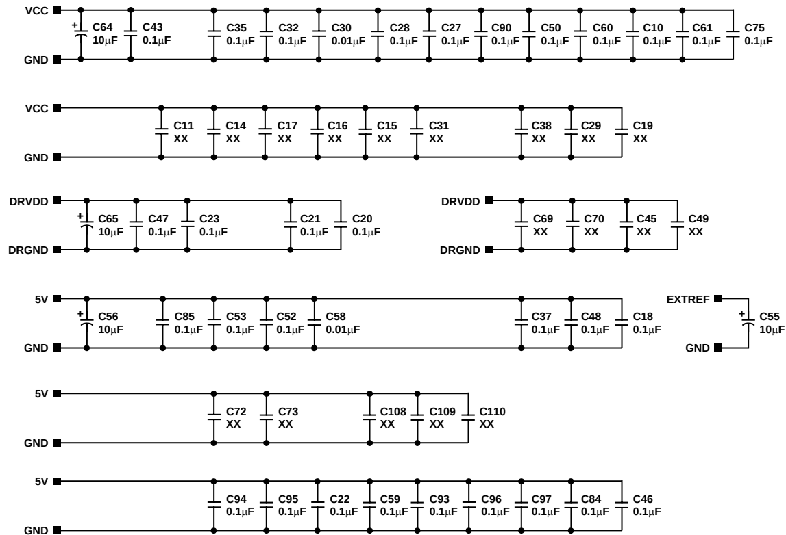
Figure 69. AD9445 Evaluation Board Schematic (Continued)
