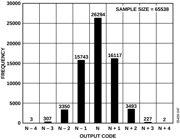
Figure 45. AD9445-105 Grounded Input Histogram
