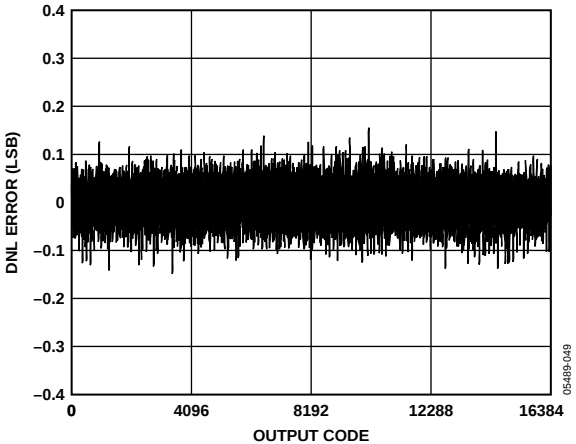
Figure 47. AD9445-105 DNL Error vs. Output Code, 105 MSPS, 10.3 MHz
