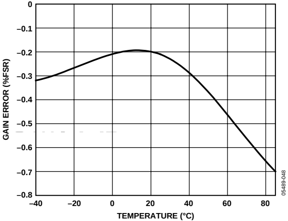
Figure 46. AD9445-125 Gain vs. Temperature
