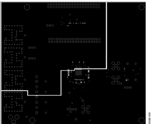
Figure 53. LVDS Mode Evaluation Board Layout, Ground Plane 1
