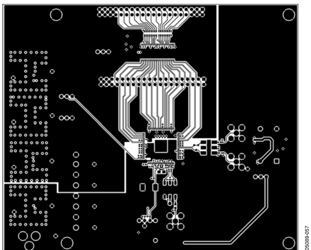
Figure 51. LVDS Mode Evaluation Board Layout, Primary Side
