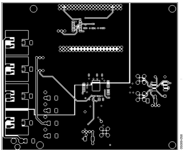
Figure 52. LVDS Mode Evaluation Board Layout, Secondary Side
