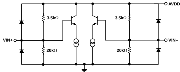
Figure 7. Analog Inputs
