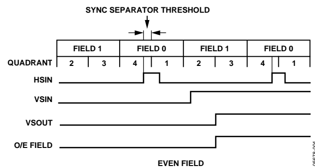
Figure 4. VSYNC Filter—Even
