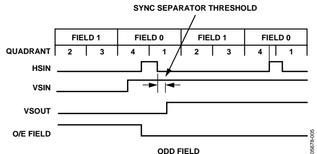
Figure 5. VSYNC Filter—Odd
