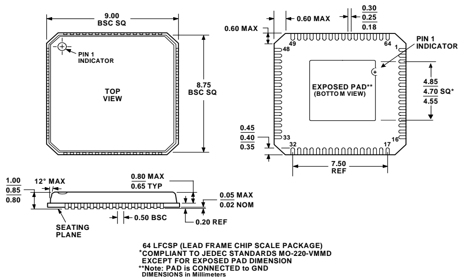
Figure 5. 64-Lead Lead Frame Chip Scale Package [LFCSP_VQ]
