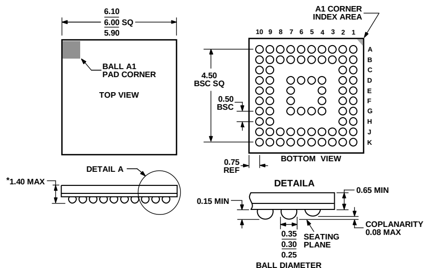
Figure 5. 76-Ball Chip Scale Package Ball Grid Array [CSP_BGA] 6 mm × 6 mm × 1.4 mm (BC-76)
