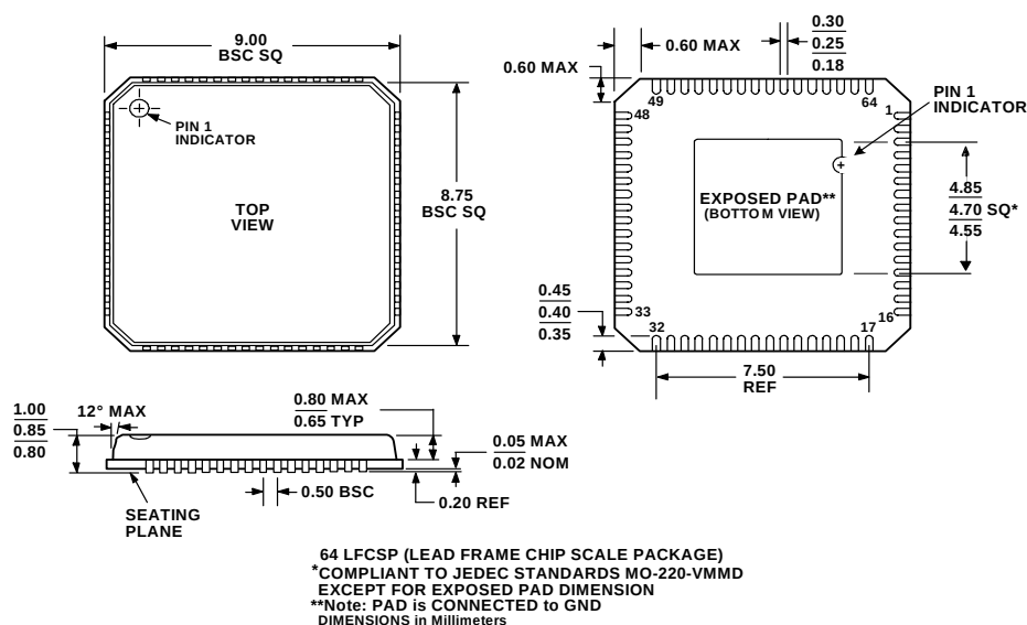
Figure 4. 64-Lead Lead Frame Chip Scale Package [LFCSP] (CP-64)
