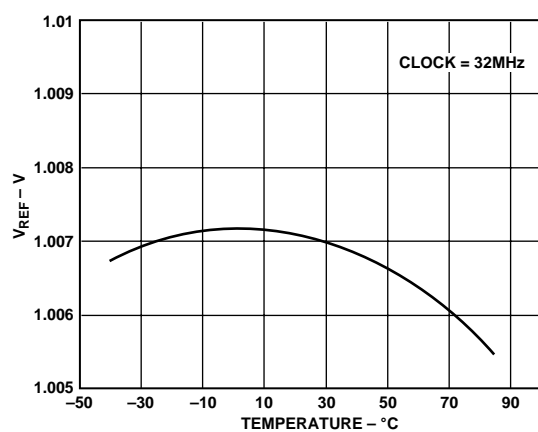
Figure 9. Voltage Reference Error vs. Temperature
