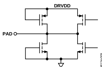
Figure 57. Digital Output
