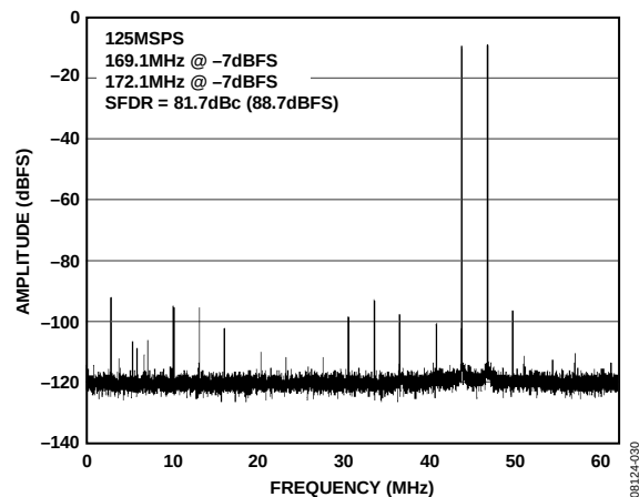
Figure 49. AD9258-125 Two-Tone FFT with f_{IN1} = 169.1 MHz and f_{IN2} = 172.1 MHz
