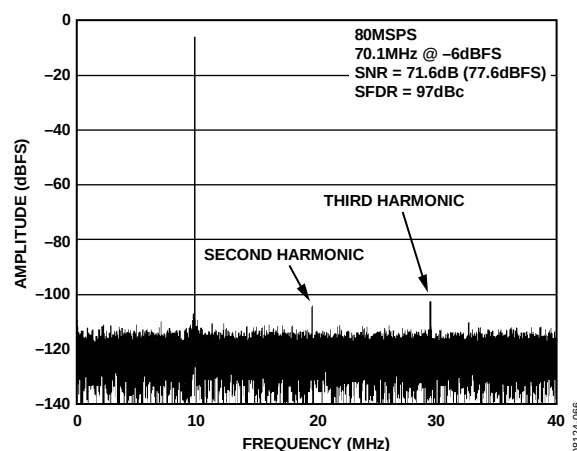
Figure 12. AD9258-80 Single-Tone FFT with f_{IN} = 70.1 MHz with Dither Enabled
