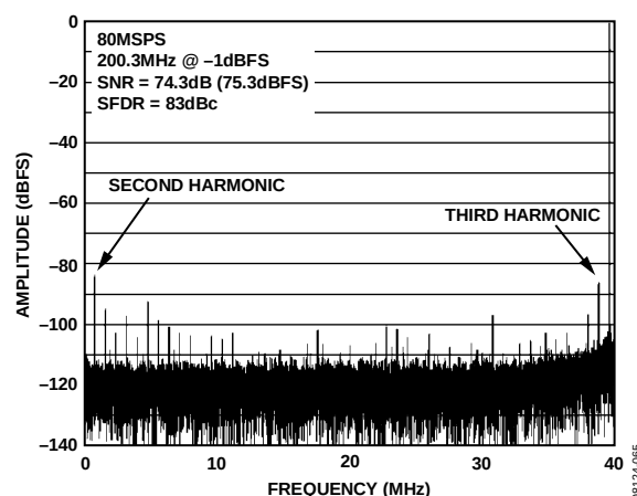
Figure 11. AD9258-80 Single-Tone FFT with f_{IN} = 200.1 MHz
