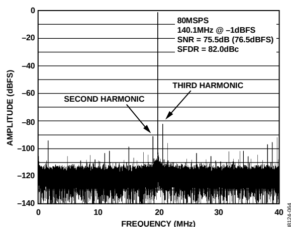
Figure 10. AD9258-80 Single-Tone FFT with f_{IN} = 140.1 MHz
