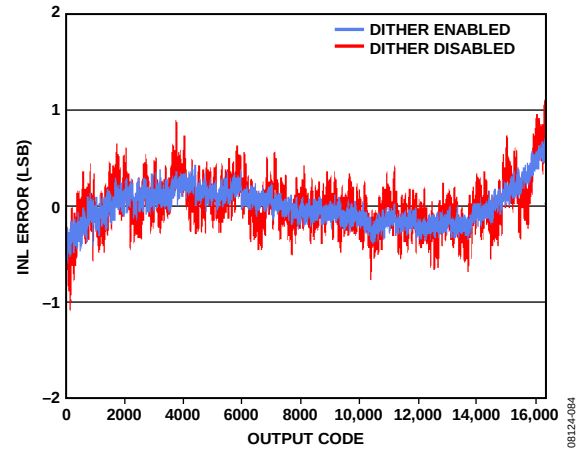
Figure 30. AD9258-105 INL with f_{IN} = 9.7 MHz
