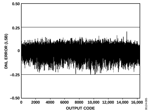
Figure 31. AD9258-105 DNL with f_{IN} = 9.7 MHz
