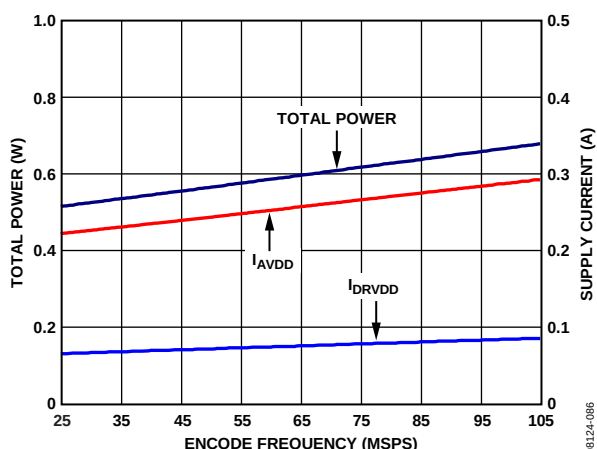
Figure 82. AD9258-105 Power and Current vs. Encode Frequency (LVDS Output Mode)
