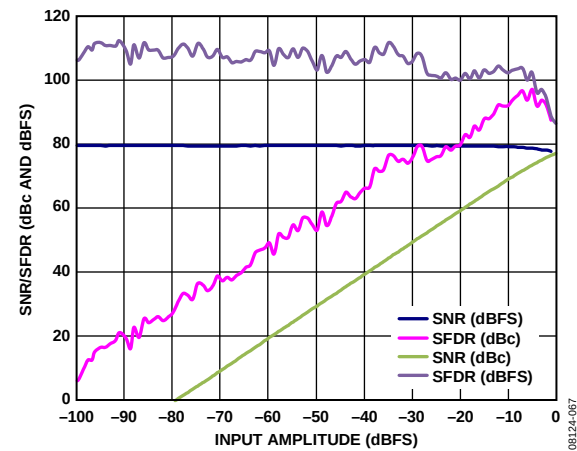
Figure 13. AD9258-80 Single-Tone SNR/SFDR vs. Input Amplitude ( A_{IN} ) with f_{IN} = 98.12 MHz
