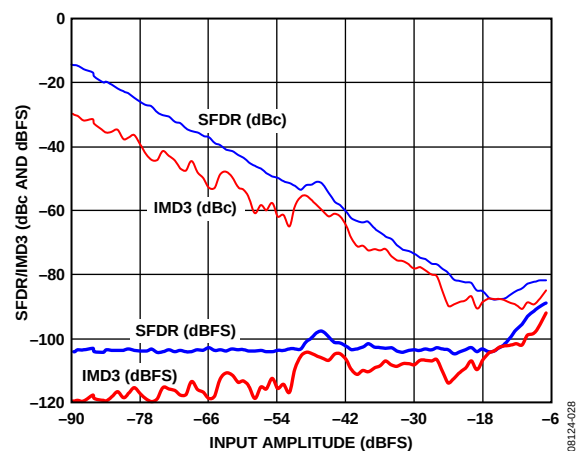
Figure 47. AD9258-125 Two-Tone SFDR/IMD3 vs. Input Amplitude ( A_{IN} ) with f_{IN1} = 169.1 MHz, f_{IN2} = 172.1 MHz, f_s = 125 MSPS
