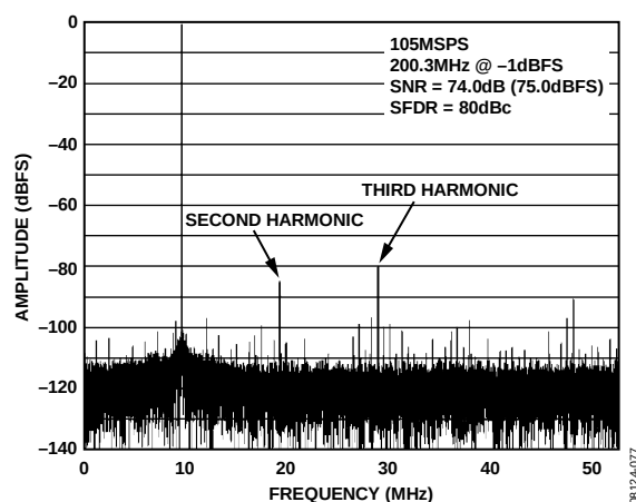
Figure 23. AD9258-105 Single-Tone FFT with f_{IN} = 200.3 MHz
