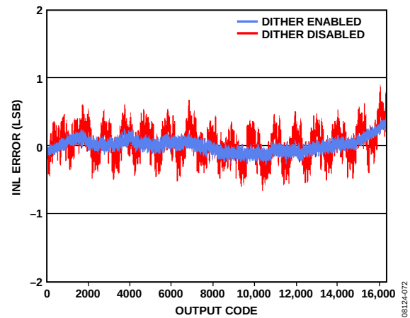
Figure 18. AD9258-80 INL with f_{IN} = 9.7 MHz
