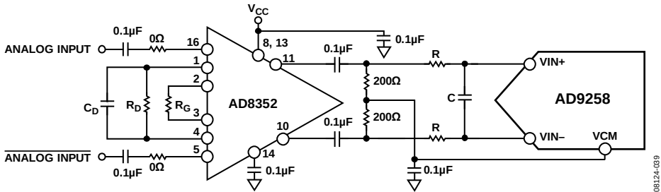
Figure 69. Differential Input Configuration Using the AD8352
