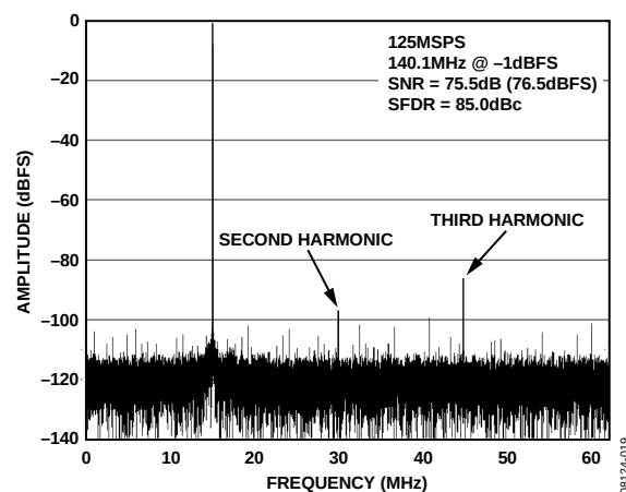
Figure 35. AD9258-125 Single-Tone FFT with f_{IN} = 140.1 MHz
