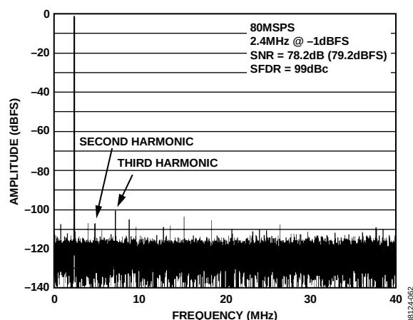
Figure 8. AD9258-80 Single-Tone FFT with f_{IN} = 2.4 MHz
