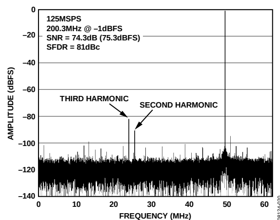
Figure 36. AD9258-125 Single-Tone FFT with f_{IN} = 200.3 MHz
