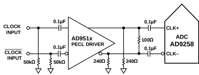
Figure 77. Differential PECL Sample Clock (Up to 625 MHz)
