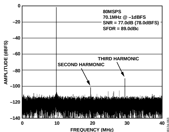
Figure 9. AD9258-80 Single-Tone FFT with f_{IN} = 70.1 MHz
