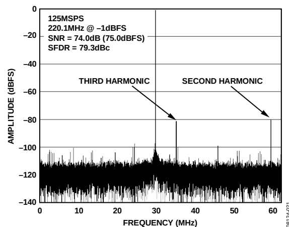
Figure 37. AD9258-125 Single-Tone FFT with f_{IN} = 220.1 MHz
