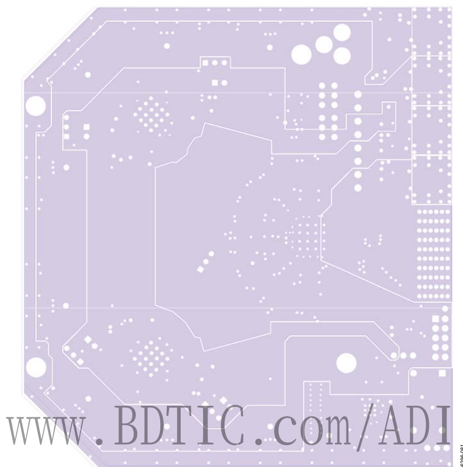
Figure 71. Evaluation Board Layout, Power Plane
