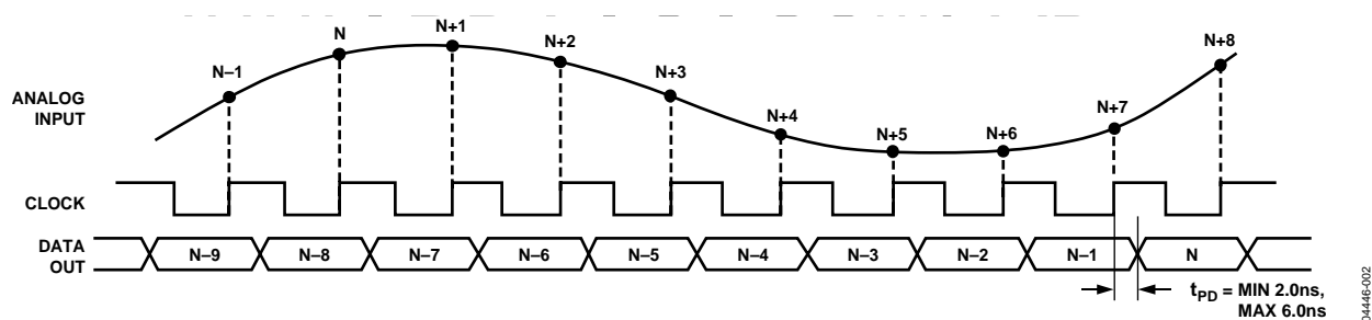
Figure 2. Timing Diagram
