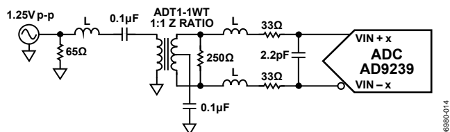
Figure 48. Differential Transformer-Coupled Configuration for Wideband IF Applications
