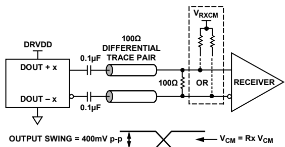
Figure 62. AC-Coupled Digital Output Termination Example
