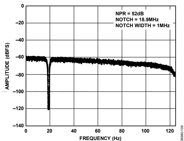
Figure 32. Noise Power Ratio (NPR), f_{SAMPLE} = 250 MSPS
