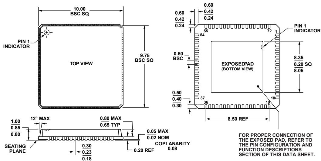
Figure 80. 72-Lead Lead Frame Chip Scale Package [LFCSP_VQ] 10 mm x 10 mm Body, Very Thin Quad (CP-72-3) Dimensions shown in millimeters
