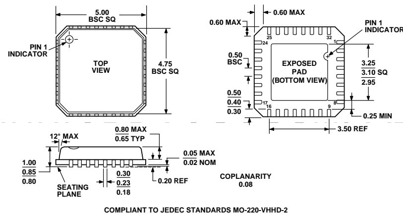
Figure 64. 32-Lead Lead Frame Chip Scale Package [LFCSP] 5 mm × 5 mm Body (CP-32-2) Dimensions shown in millimeters
