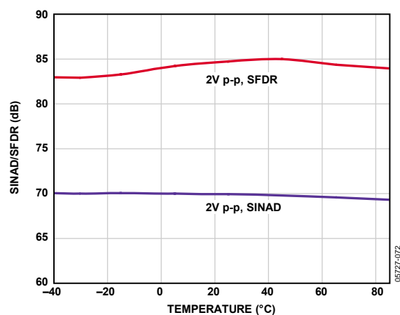
Figure 36. SINAD/SFDR vs. Temperature, f_{IN} = 10.3 MHz, f_{SAMPLE} = 65 MSPS
