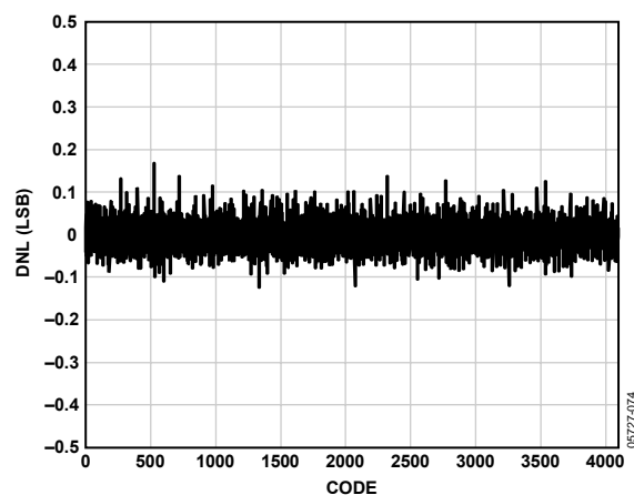
Figure 38. DNL, f_{IN} = 2.4 MHz, f_{SAMPLE} = 65 MSPS
