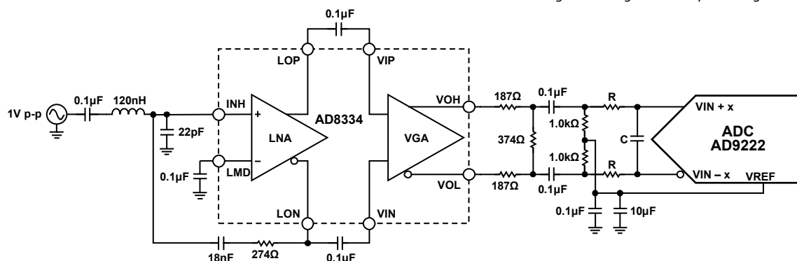
Figure 62. Differential Input Configuration Using the AD8334
