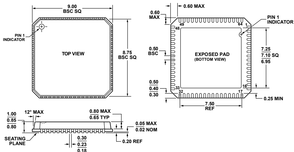
Figure 101. 64-Lead Lead Frame Chip Scale Package [LFCSP_VQ] 9 mm × 9 mm Body, Very Thin Octal (CP-64-3) Dimensions shown in millimeters
