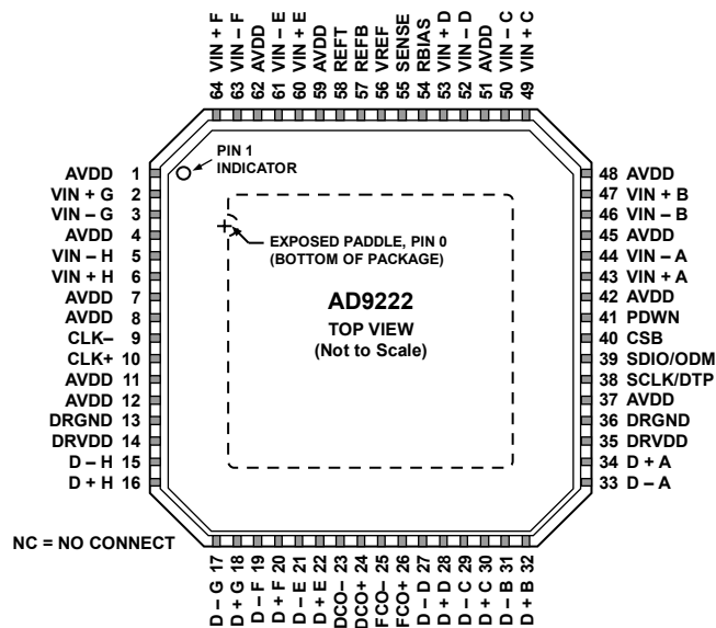
Figure 5. 64-Lead LFCSP Pin Configuration, Top View
