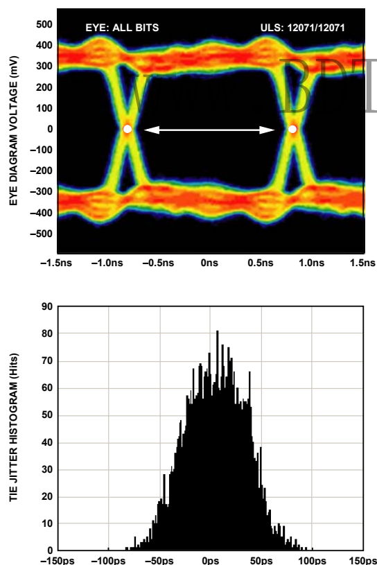
Figure 73. Data Eye for LVDS Outputs in ANSI-644 Mode with Trace Lengths Less than 24 Inches on Standard FR-4, AD9222-50
