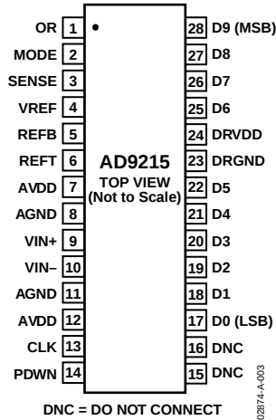
Figure 3. TSSOP (RU-28)
