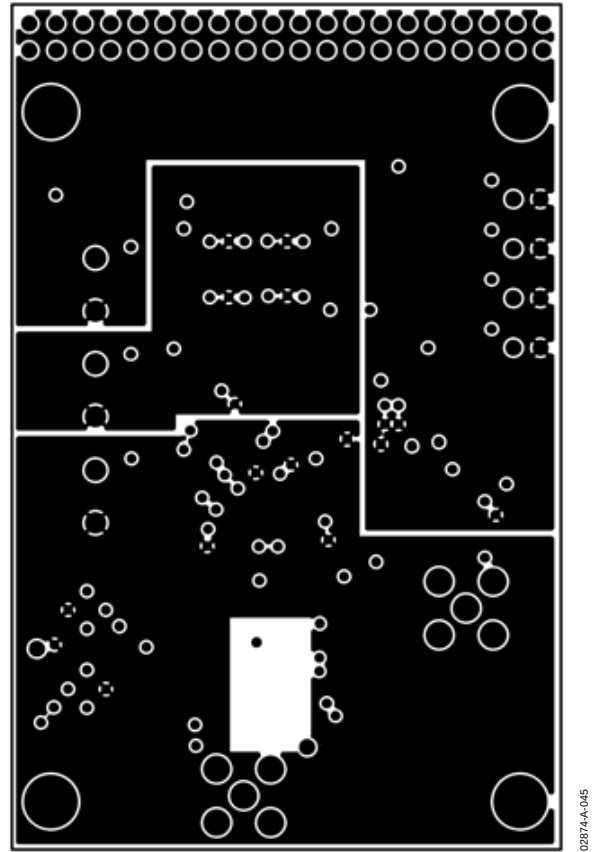
Figure 47. LFCSP Evaluation Board Layout, Power Plane
