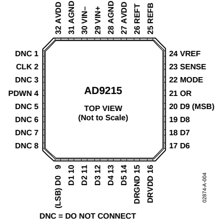
Figure 4. LFCSP (CP-32)
