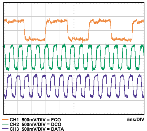
Figure 59. LVDS Output Timing Example in ANSI-644 Mode (Default), AD9212-65
