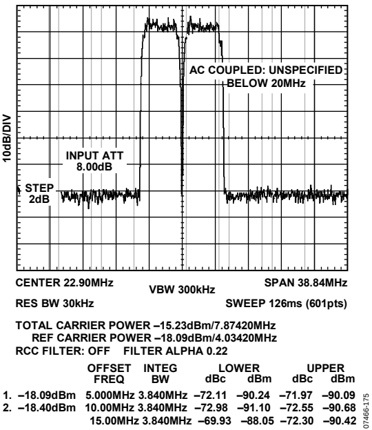
Figure 75. AD9117 ACLR Two-Carrier, 3.3 V
