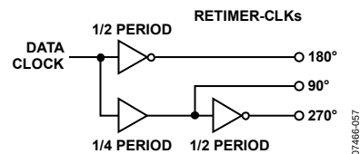
Figure 95. RETIMER-CLK Phases
