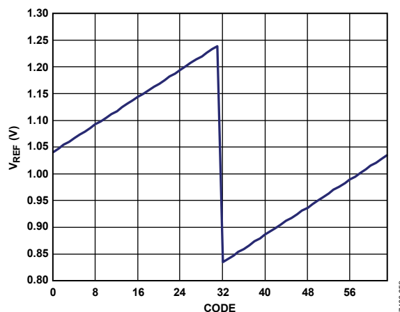
Figure 97. Typical V_{REF} Voltage vs. Code
