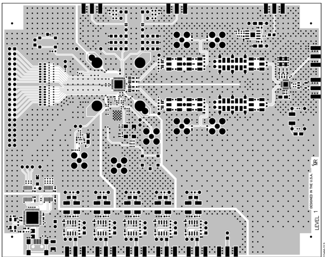
Figure 130. Layer 1—Primary Side
