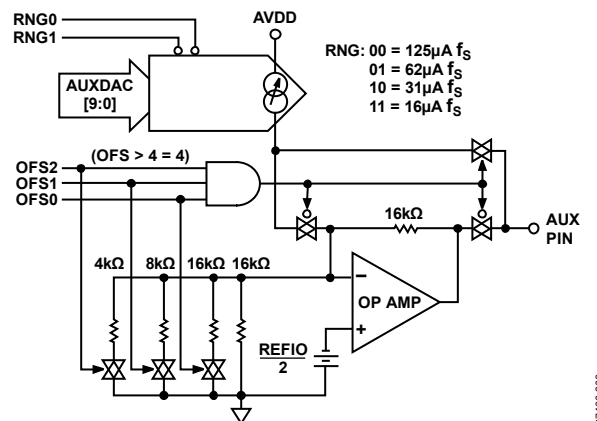
Figure 105. AUXDAC Simplified Circuit Diagram
