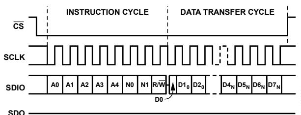
Figure 88. Serial Register Interface Timing, LSB First Read
