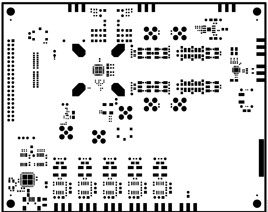
Figure 133. Solder Mask—Primary Side, No Socket
