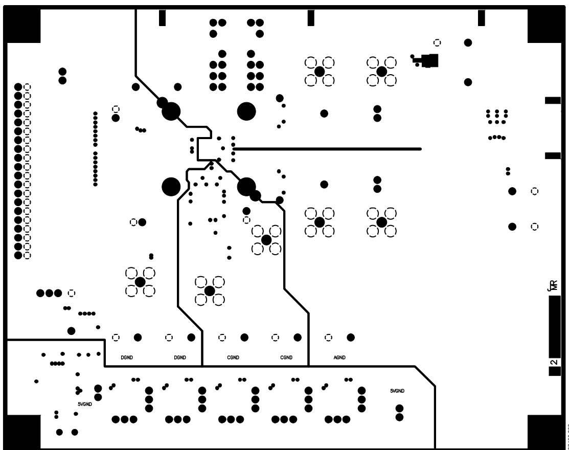
Figure 119. Layer 2, Ground Plane
