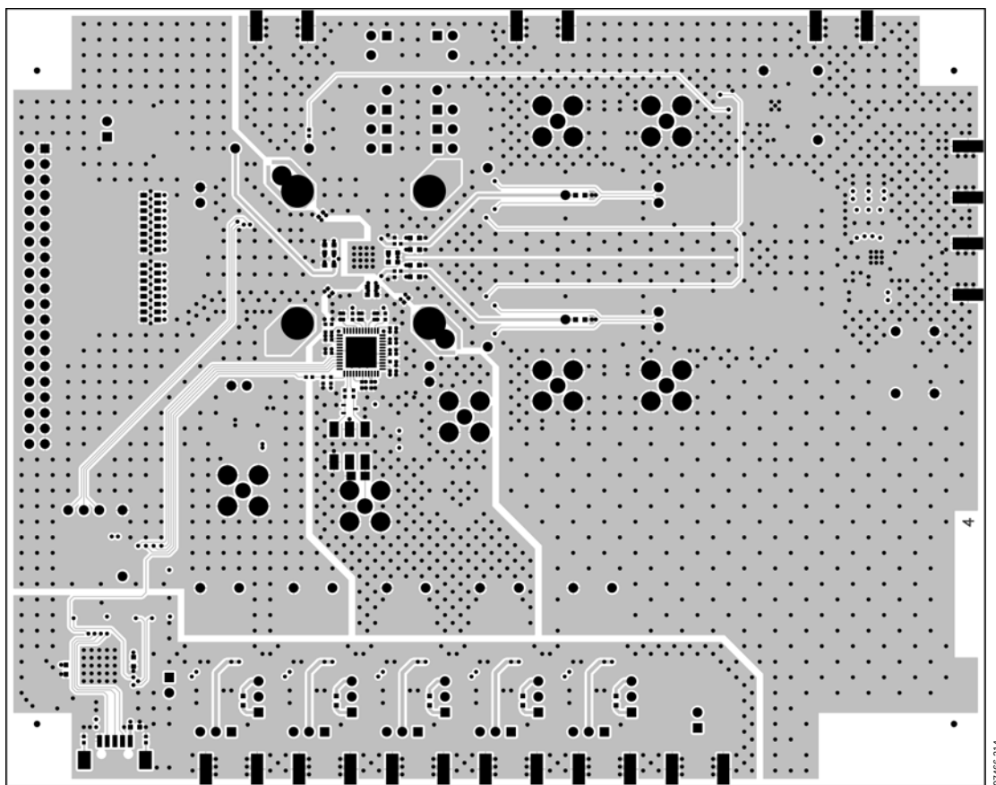
Figure 131. Layer 4—Secondary Side
