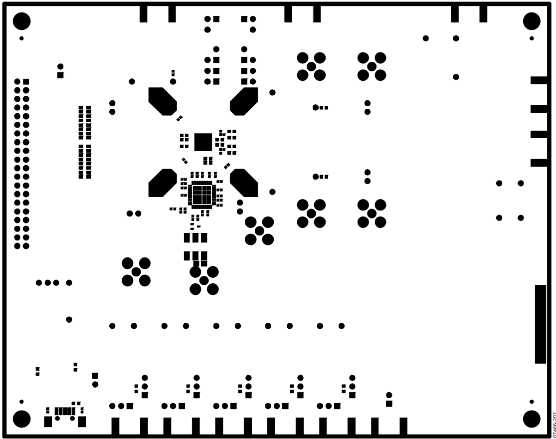
Figure 124. Solder Mask—Secondary Side
