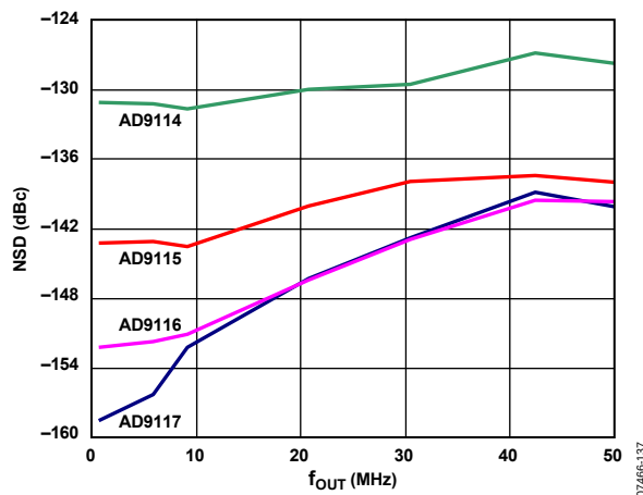
Figure 37. NSD at 8 mA vs. f_{OUT} , 1.8 V
