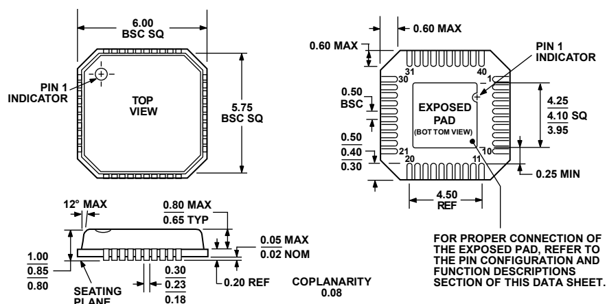
Figure 134. 40-Lead Lead Frame Chip Scale Package [LFCSP_VQ] 6 mm x 6 mm, Very Thin Quad (CP-40-1) Dimensions shown in millimeters
