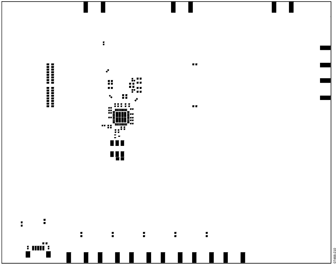
Figure 127. Secondary Side Paste
