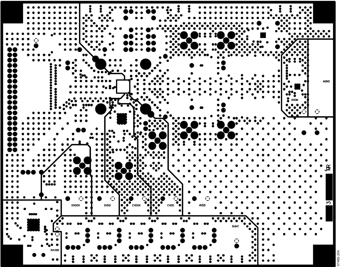
Figure 120. Layer 3, Power Plane
