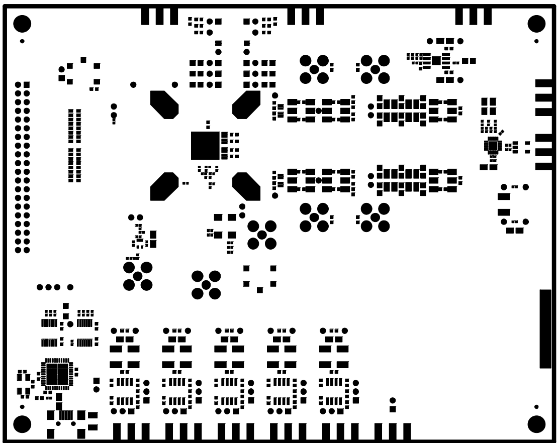
Figure 123. Solder Mask—Primary Side with Socket
