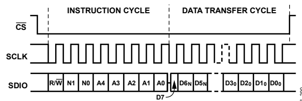
Figure 86. Serial Register Interface Timing, MSB First Read
