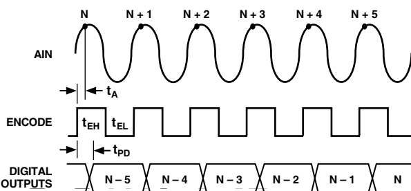
Figure 1. Timing Diagram
