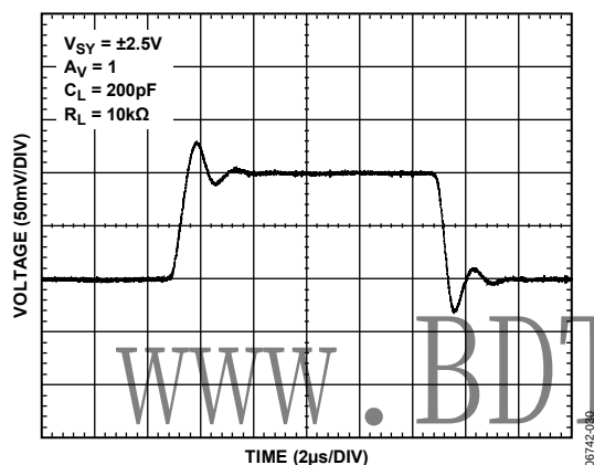
Figure 30. Small Signal Transient Response, V_{SV} = \pm 2.5V
