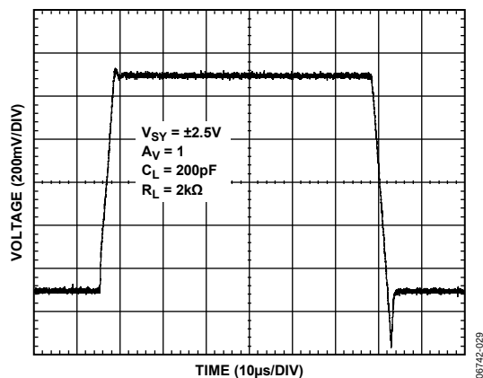
Figure 29. Large Signal Transient Response, V_{SV} = \pm 2.5V
