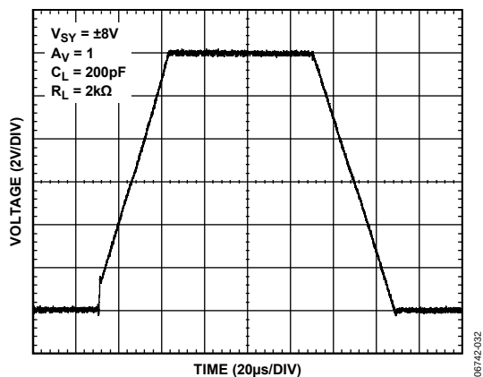
Figure 32. Large Signal Transient Response, V_{SV} = \pm 8V
