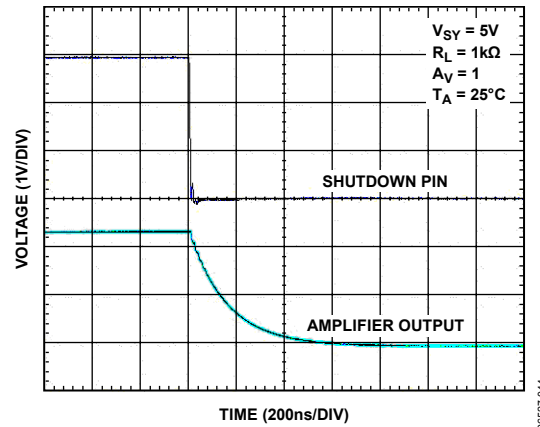
Figure 45. Turn-Off Time
