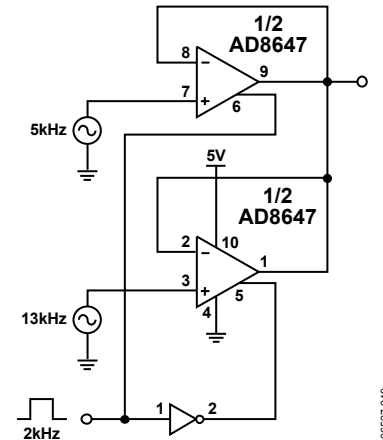
Figure 48. AD8647 Output Switching
