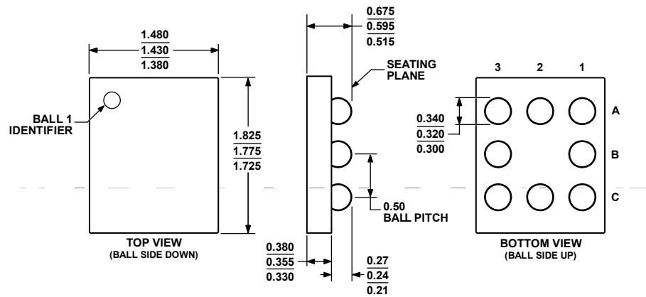
Figure 61. 8-Ball Wafer Level Chip Scale Package [WL CSP] (CB-8-1)
