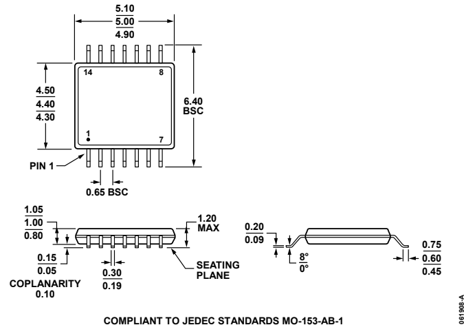
Figure 63. 14-Lead Thin Shrink Small Outline Package [TSSOP] (RU-14)
