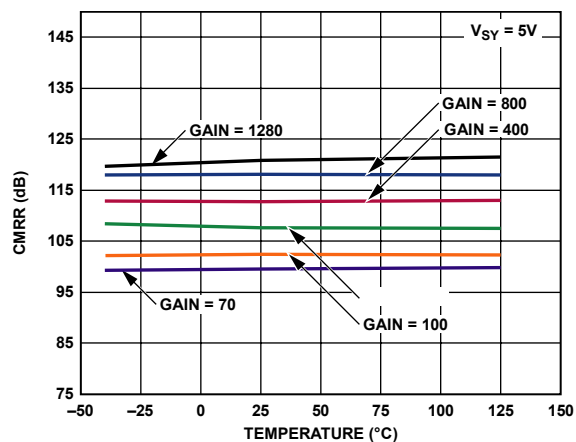
Figure 18. CMRR vs. Temperature at Different Gains
