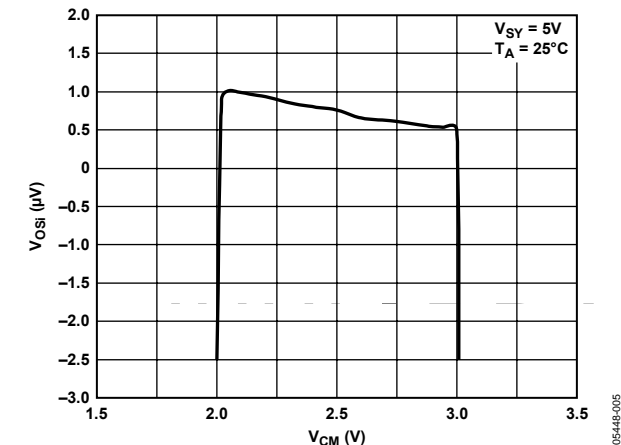
Figure 5. Input Offset Voltage vs. Common-Mode Voltage
