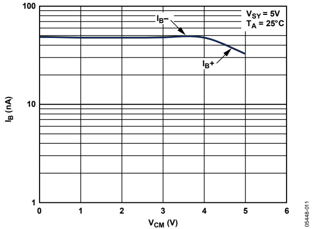
Figure 10. Input Bias Current at VPOS, VNEG vs. Common-Mode Voltage
