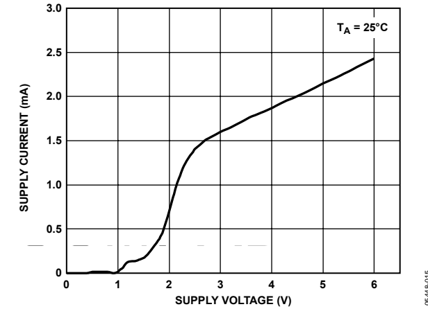
Figure 14. Supply Current ( I_{SY} ) vs. Supply Voltage
