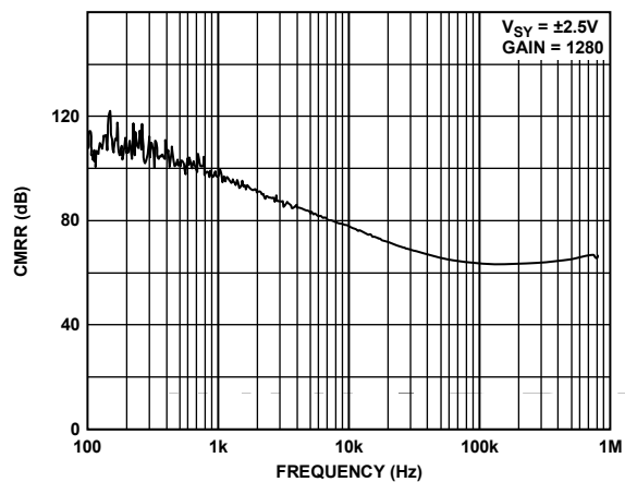
Figure 17. CMRR vs. Frequency
