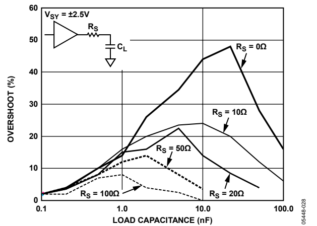
Figure 27. Output Buffer Negative Overshoot
