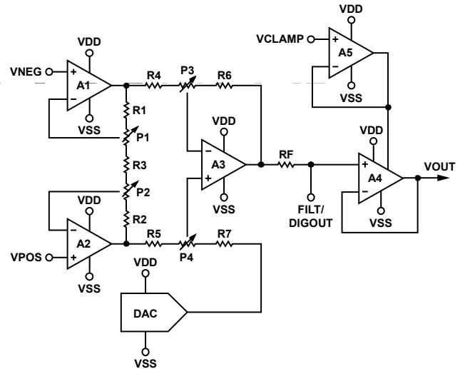
Figure 47. Functional Schematic
