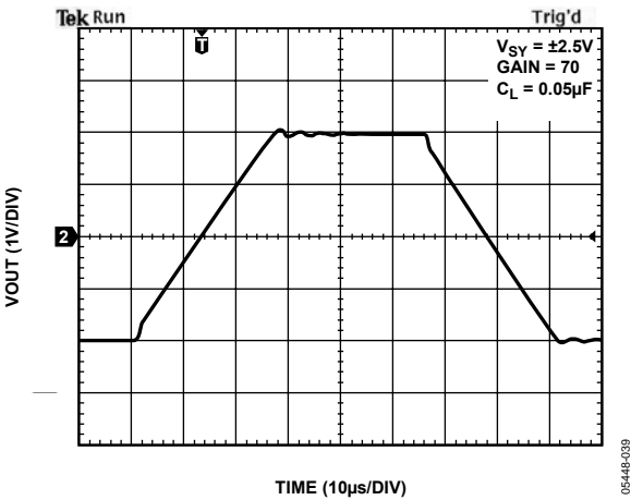
Figure 38. Large Signal Response at C_L = 0.05 \mu F
