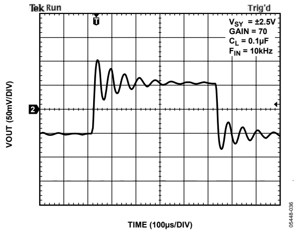
Figure 35. Small Signal Response at C_L = 0.1 \mu F and F_{IN} = 10 \text{ kHz}
