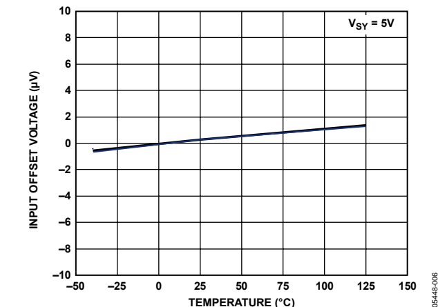
Figure 6. Input Offset Voltage vs. Temperature
