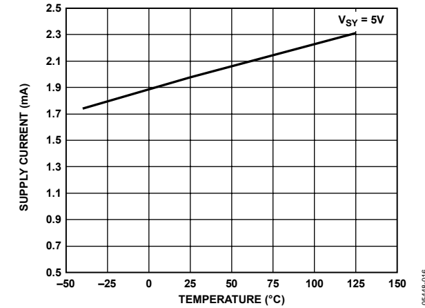
Figure 15. Supply Current ( I_{SY} ) vs. Temperature
