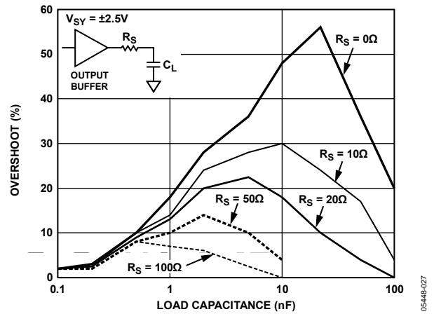
Figure 26. Output Buffer Positive Overshoot
