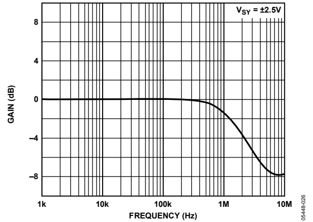
Figure 25. Output Buffer Gain vs. Frequency
