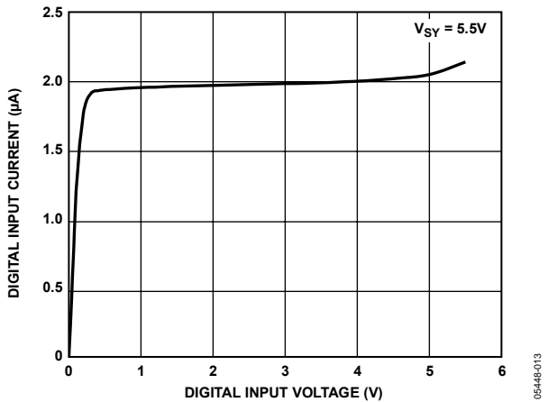
Figure 12. Digital Input Current vs. Digital Input Voltage (Pin 4)
