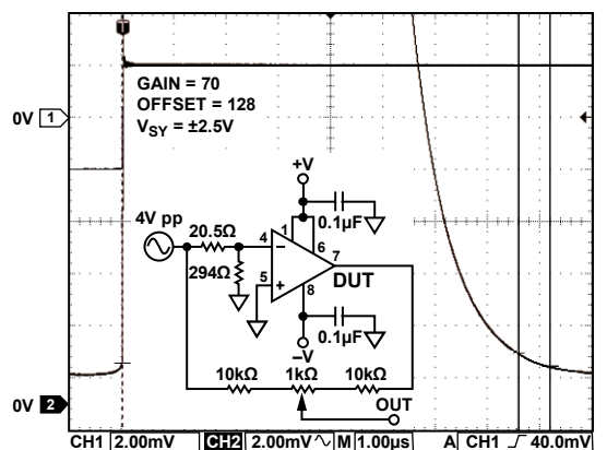
Figure 45. Settling Time 0.01%
