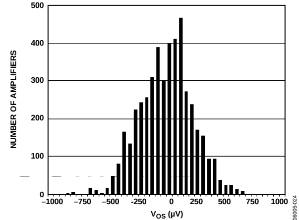
Figure 24. Input Offset Voltage Distribution ( 0 V < V_{CM} < 1.8 V)
