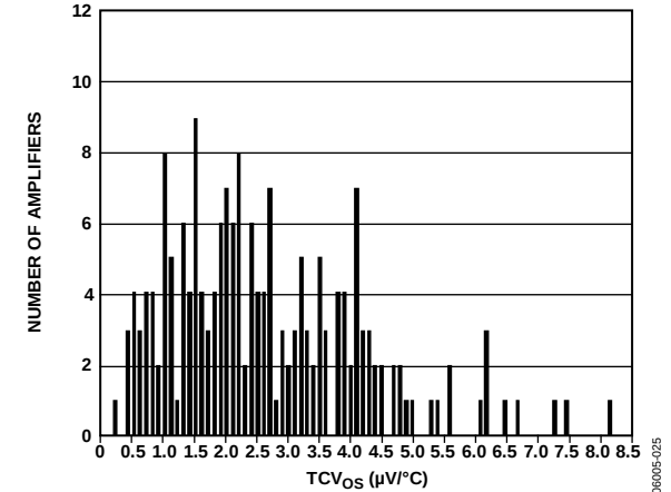
Figure 25. Input Offset Voltage Drift Distribution ( -40^{\circ} C < T_A < +85^{\circ} C)
