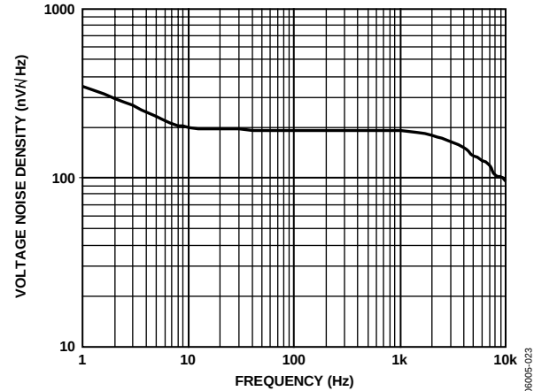
Figure 23. Voltage Noise Density ( V_S = 1.8 V and 5.0 V)
