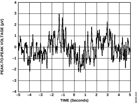
Figure 22. 0.1 Hz to 10 Hz Input Voltage Noise ( V_S = 5 V and 1.8 V)
