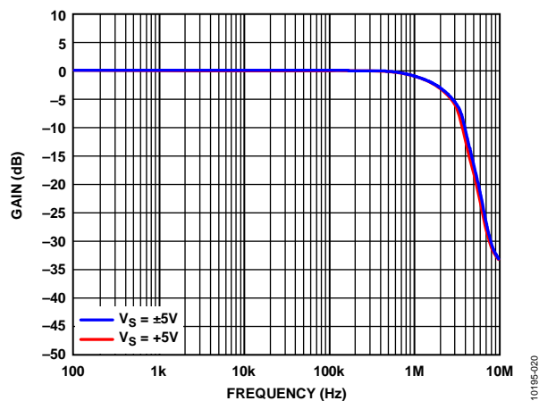
Figure 18. Large Signal Frequency Response for Various Supplies
