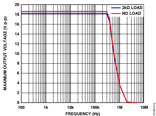
Figure 9. Maximum Output Voltage vs. Frequency
