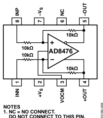
Figure 49. Block Diagram
