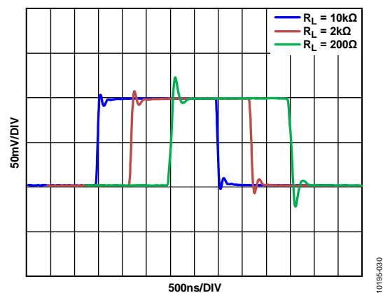
Figure 27. Small Signal Step Response for Various Resistive Loads, V_S = \pm 5V
