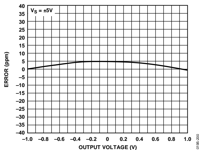
Figure 42. Gain Nonlinearity
