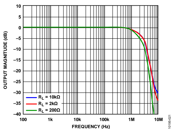
Figure 19. Large Signal Frequency Response for Various Loads
