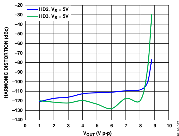
Figure 38. Harmonic Distortion vs. V_{OUT,dm} f = 10 kHz
