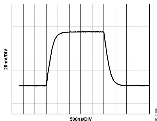
Figure 29. VOCM Small Signal Step Response
