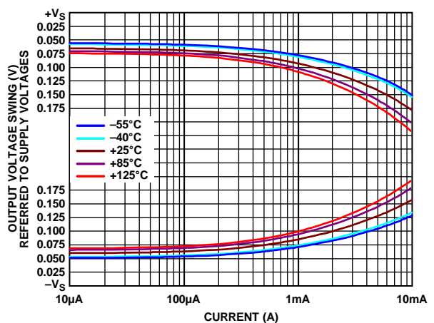
Figure 13. Output Voltage Swing vs. Load Current vs. Temperature, V_S = \pm 5\text{ V}
