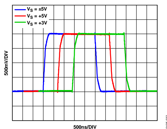
Figure 26. Large Signal Pulse Response for Various Supplies
