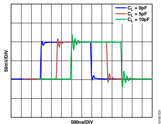
Figure 28. Small Signal Step Response for Various Capacitive Loads, V_S = \pm 5V
