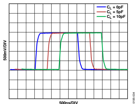
Figure 31. Large Signal Step Response for Various Capacitive Loads, V_S = \pm 5V
