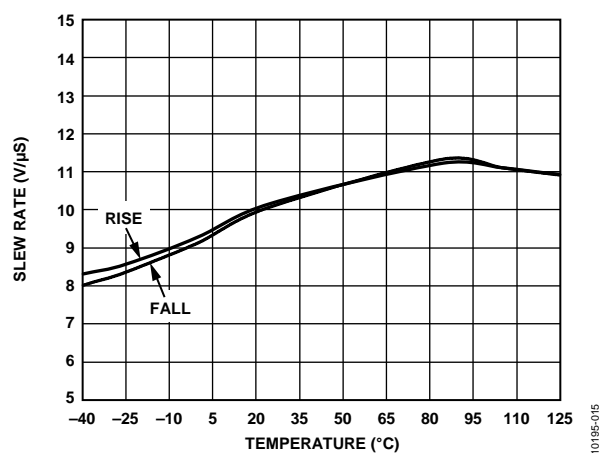
Figure 11. Slew Rate vs. Temperature
