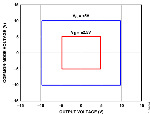
Figure 6. Input Common-Mode Voltage vs. Output Voltage, V_S = \pm 5\text{ V} and \pm 2.5\text{ V}
