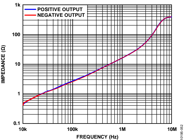
Figure 47. Output Impedance vs. Frequency
