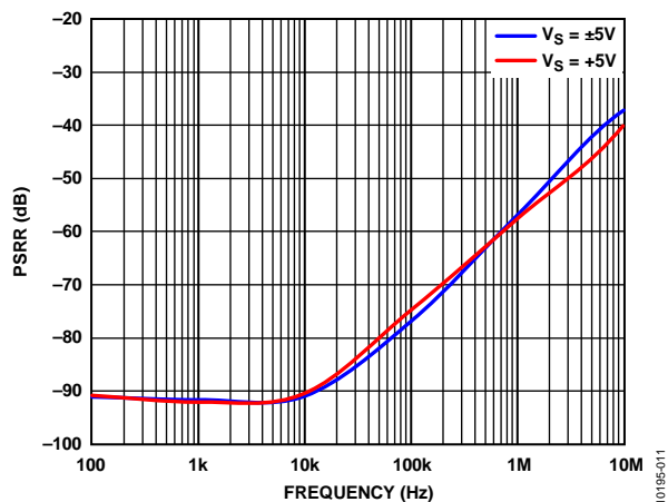
Figure 8. Power Supply Rejection vs. Frequency
