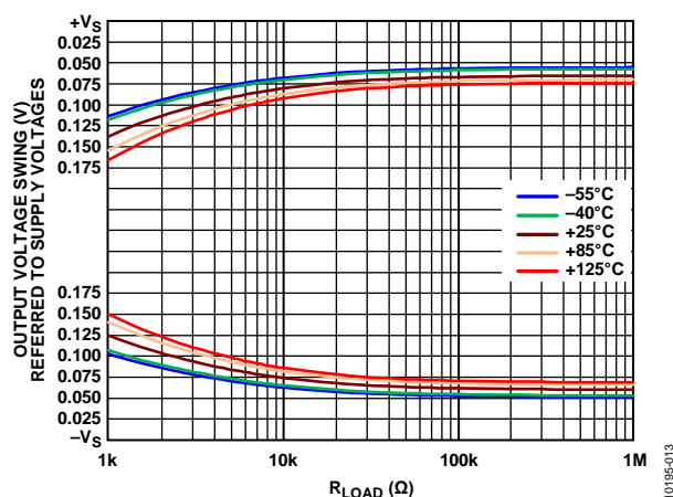
Figure 10. Output Voltage Swing vs. R_{LOAD} vs. Temperature, V_S = \pm 5\text{ V}
