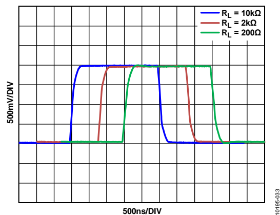
Figure 30. Large Signal Step Response for Various Resistive Loads, V_S = \pm 5V
