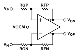
Figure 50. Functional Circuit Diagram of the AD8476 at a Given Gain
