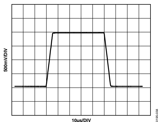
Figure 32. VOCM Large Signal Step Response
