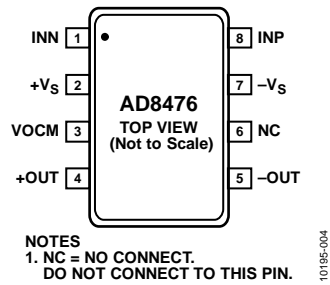
Figure 2. 8-Lead MSOP Pin Configuration
