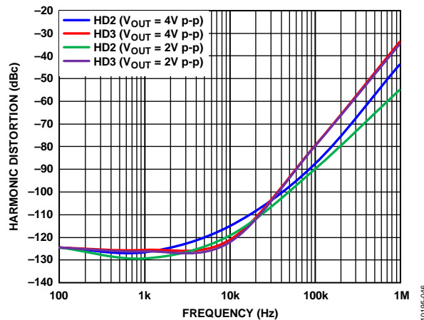
Figure 37. Harmonic Distortion vs. Frequency at Various V_{OUT,dm}
