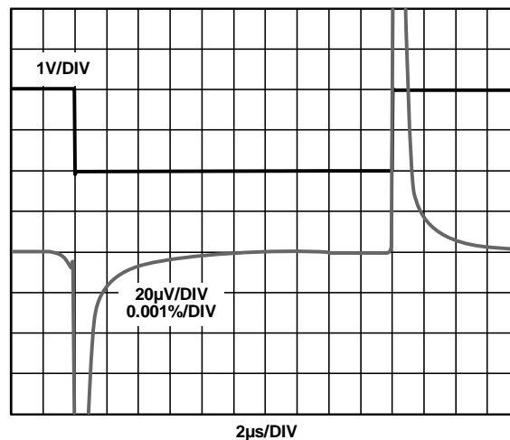
Figure 44. Settling Time to 0.001% of 2 V Step
