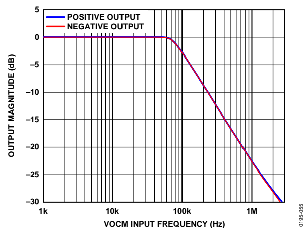
Figure 25. V OCM Large Signal Frequency Response
