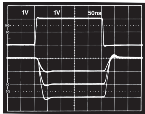
Figure 16. VGA Transient Response with V_X = 1\text{ V} , 2\text{ V} , and 3\text{ V}
