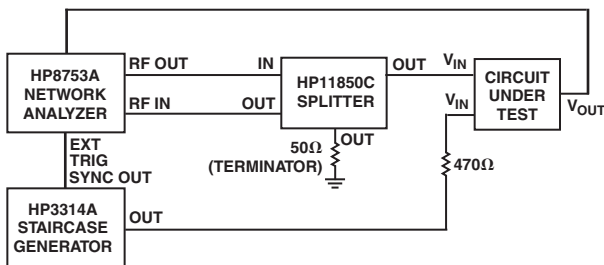
Figure 11b. Differential Gain/Phase Test Setup
