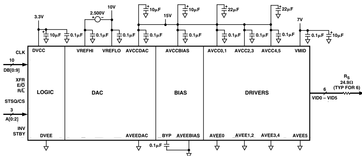
Figure 10. Interface Drawing
