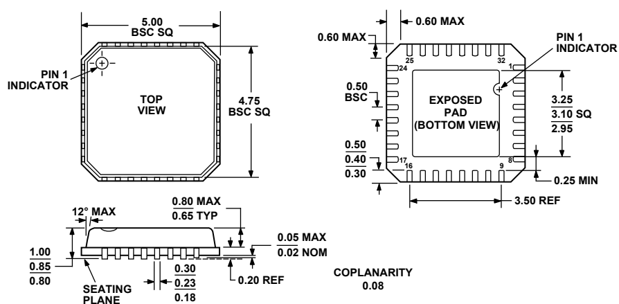
COMPLIANT TO JEDEC STANDARDS MO-220-VHHD-2 Figure 52. 32-Lead Lead Frame Chip Scale Package [LFCSP_VQ] 5 mm × 5 mm Body, Very Thin Quad (CP-32-2) Dimensions shown in millimeters
