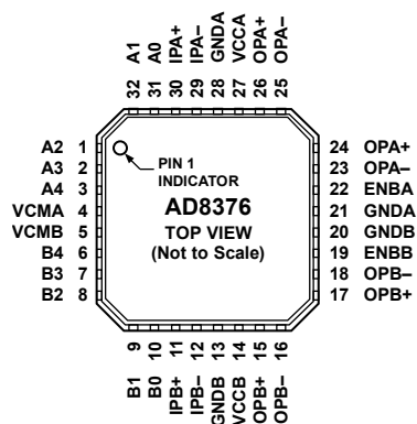
Figure 3. 32-Lead LFCSP
