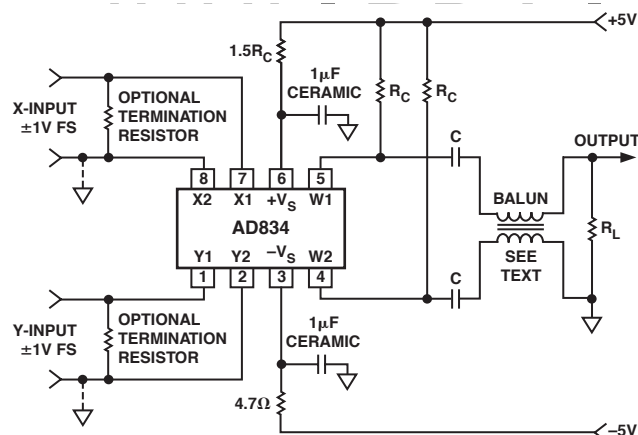
Figure 7. Using a Balun at the Output
