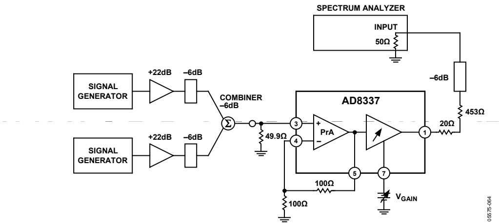
Figure 64. IMD and OIP3
