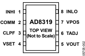
Figure 2. Pin Configuration
