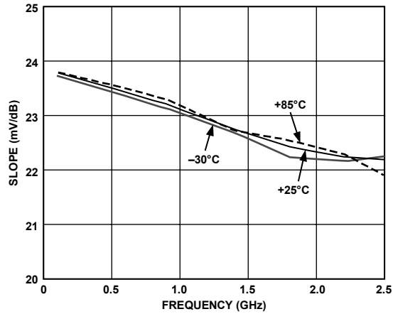
Figure 15. Slope vs. Frequency; -30°C, +25°C, and +85°C
