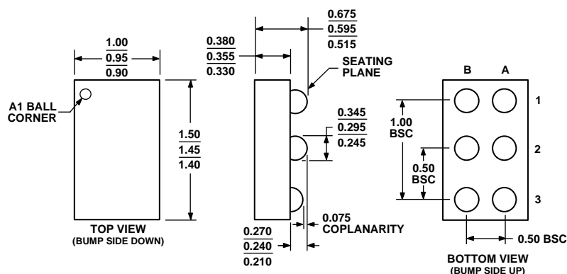
Figure 46. 6-Ball Wafer Level Chip Scale Package [WLCSP] (CB-6) Dimensions shown in millimeters
