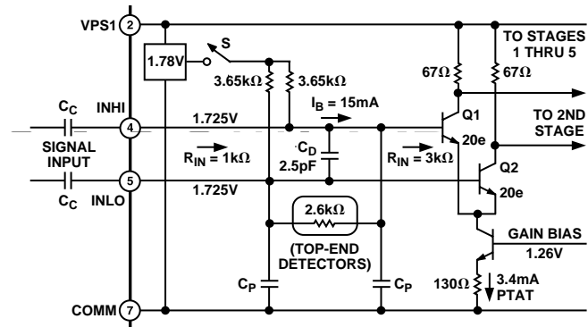
Figure 27. Signal Input Interface
