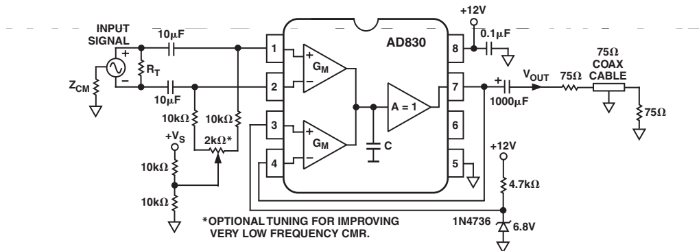
Figure 28. AC-Coupled Line Receiver
