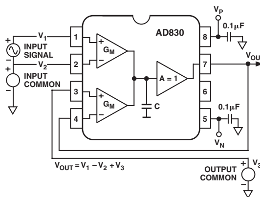
Figure 20. Differential Amplification with Level Shifting
