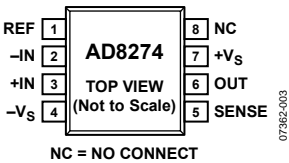
Figure 4. SOIC Pin Configuration
