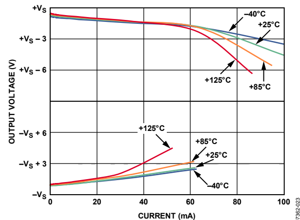
Figure 18. Output Voltage vs. I_{OUT}
