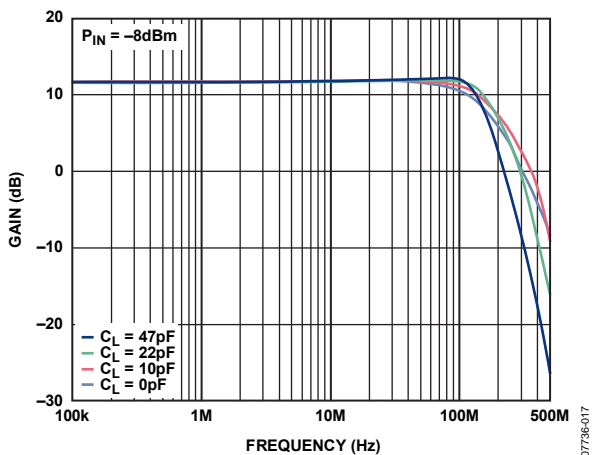
Figure 17. Large Signal Frequency Response to VGx for Various Capacitive Loads with Series R = 10\ \Omega
