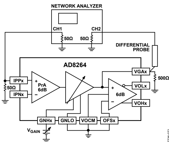
Figure 73. Frequency Response vs. Gain to V_{\text{GAx}} for Various Values of V_{\text{GAIN}} V_{\text{GAIN}} = V_{\text{GNHx}} - V_{\text{GNLx}} (See Figure 10)
