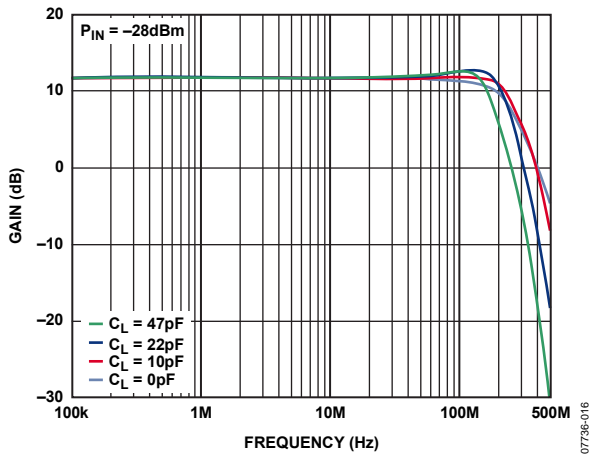
Figure 16. Small Signal Frequency Response to VGx for Various Capacitive Loads with Series R = 10\ \Omega
