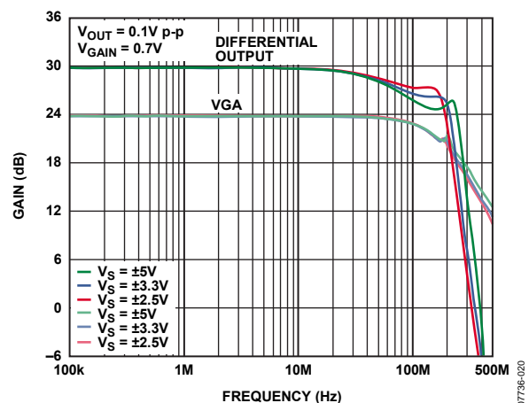
Figure 20. Large Signal Frequency Response to VGx and Differential Output for Various Supply Voltages
