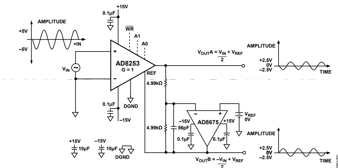
Figure 61. Differential Output with Level Shift
