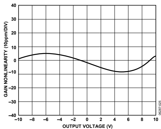
Figure 24. Gain Nonlinearity vs. Output Voltage, G = 2 , R_L = 10\text{ k}\Omega , 2\text{ k}\Omega , 600\text{ }\Omega
