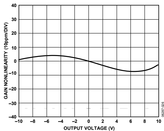
Figure 25. Gain Nonlinearity vs. Output Voltage, G = 4 , R_L = 10\text{ k}\Omega , 2\text{ k}\Omega , 600\text{ }\Omega
