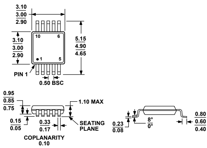
Figure 60. 10-Lead Mini Small Outline Package [MSOP] (RM-10)
