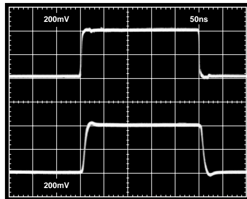
Figure 23. Noninverting Large Signal Pulse Response, R_L = 1 k\Omega
