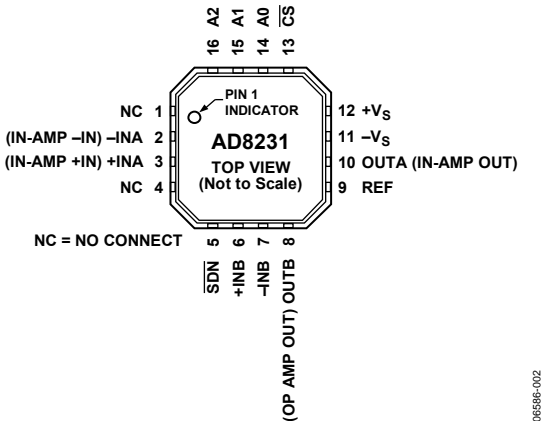
Figure 2. 16-Lead LFCSP (Chip Scale)
