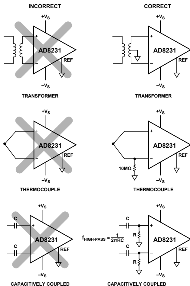
Figure 32. Creating an I_{\text{BIAS}} Path
