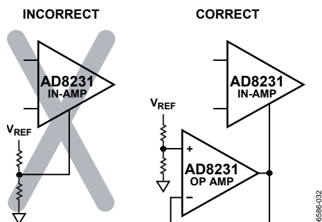
Figure 31. Driving the Reference Pin
