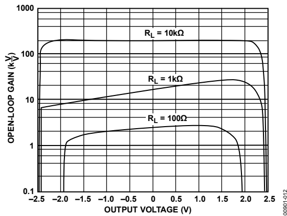
Figure 12. Open-Loop Gain vs. Output Voltage, V_S = \pm 2.5\text{ V}
