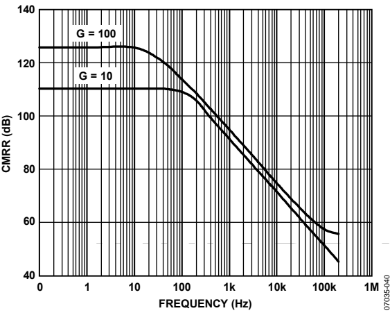
Figure 22. CMRR vs. Frequency, RTI, 1 k \Omega Source Imbalance
