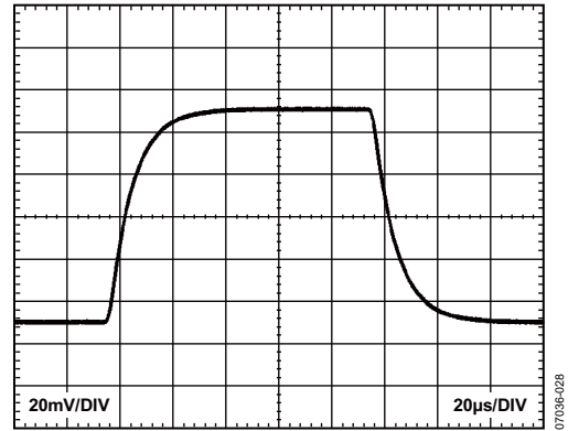
图53.小信号响应 ( G = 100 , R_L = 10\text{ k}\Omega , C_L = 100\text{ pF} )
